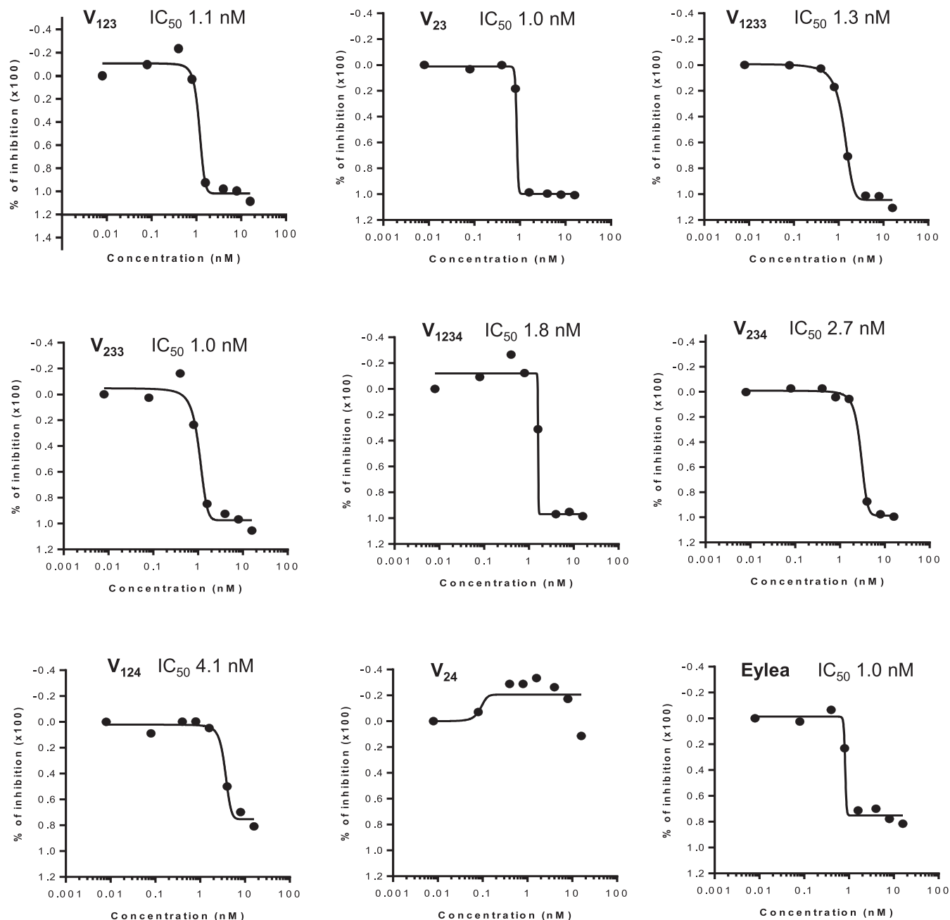
Fig. 3. IC_{50} values of the inhibitors. Bovine chorioid ECs were maintained as described in Materials and Methods . For assays, cells are plated at low density. Inhibitors were then added at various concentrations as indicated. VEGF 165 was added at the final concentration of 10 ng/mL. Cell densities were evaluated after 5 d. IC_{50} values were calculated using GraphPad Prism 5 (GraphPad Software). Data shown are based on two independent experiments obtained with highly purified proteins and are consistent with numerous previous assays.
